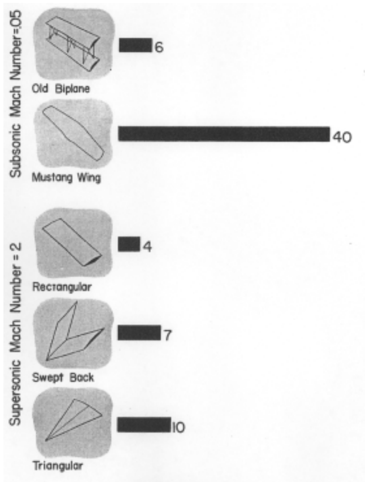
Figure 3 - Optimum Lift-Drag Ratios
