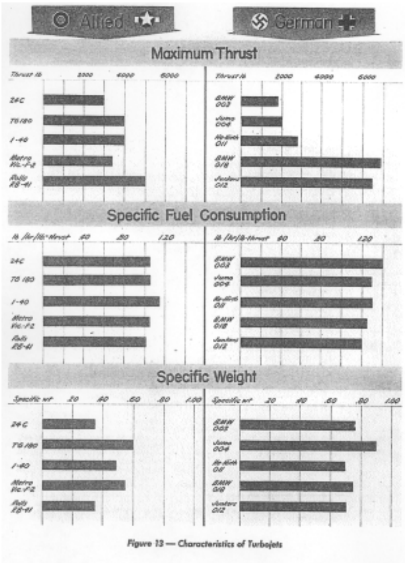
Figure 13 - Characteristics of Turbojets
