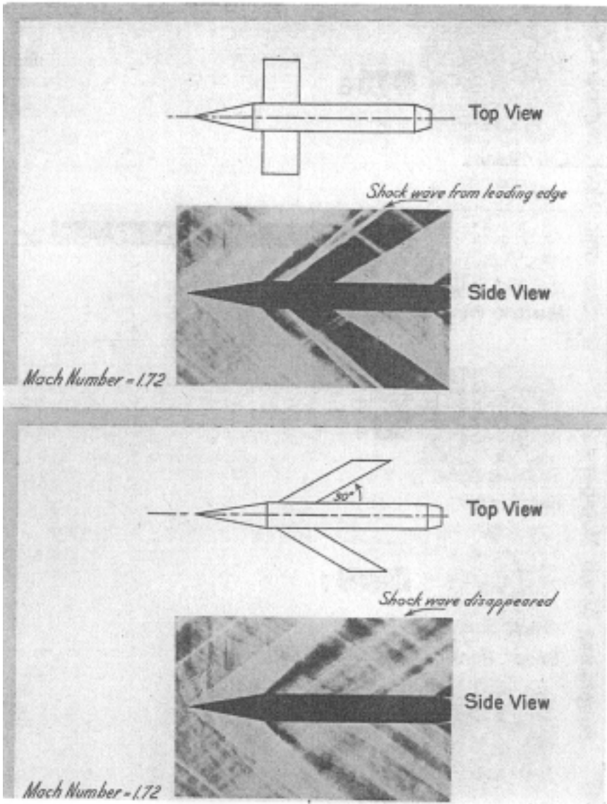
Figure 4 - Sweepback Effect on Shock Wave.
