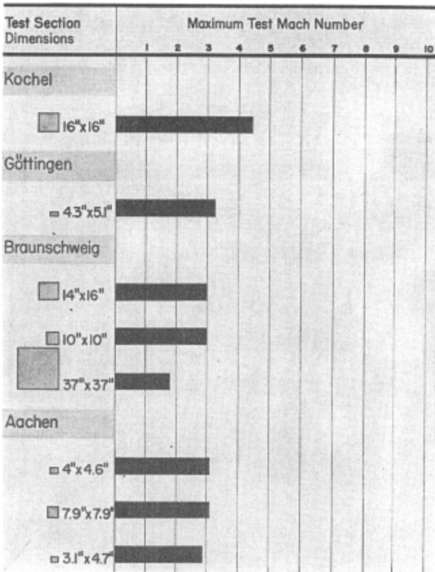
Figure 1- German Supersonic Wind Tunnels (operation 1945)
