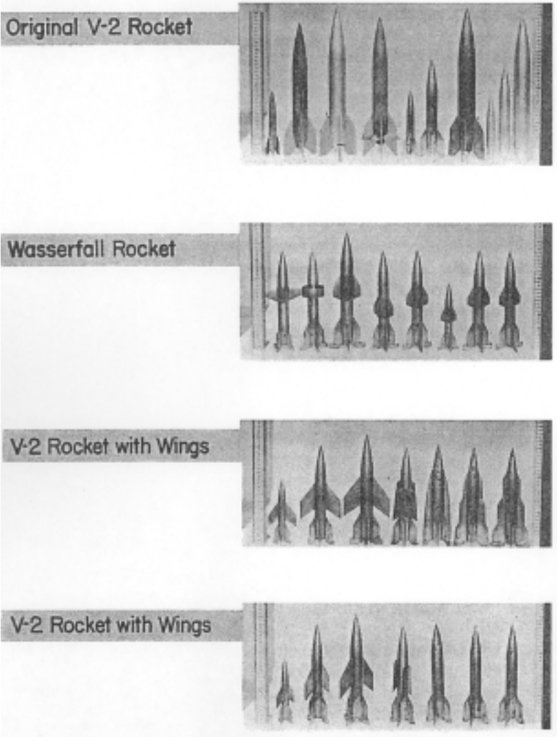
Figure 7 - Rocket Models for Supersonic Wind-Tunnel Tests
