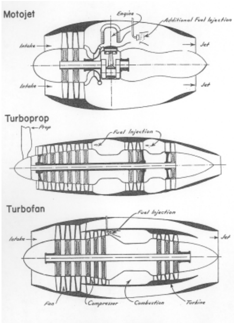
Figure 10-A - Various Propulsion Systems
