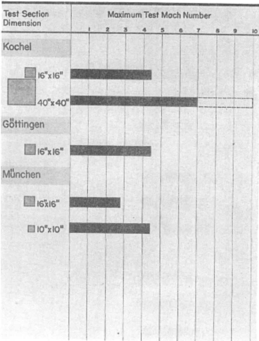
Figure 2 - German Supersonic Wind Tunnels (Construction 1945)
