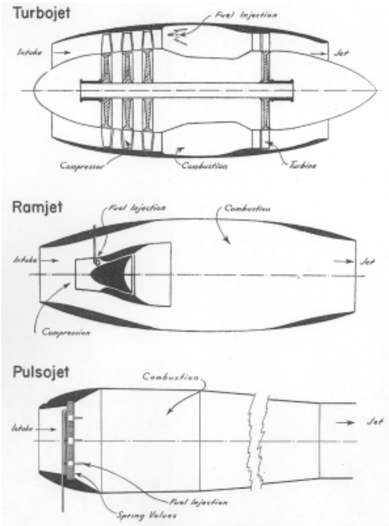
Figure 10-B - Various Propulsion Systems
